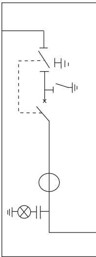
Single Isolation Cubicle Lateral Outgoing (with Circuit Breaker and Air Rotary Disconnector)
