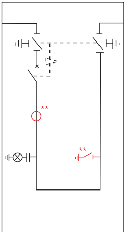
Busbar Coupling Cubicle with Air Rotary Disconnector
