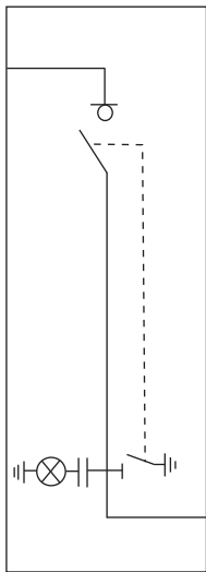
Single Isolation Cubicle Lateral Outgoing (with Switch Disconnector)
