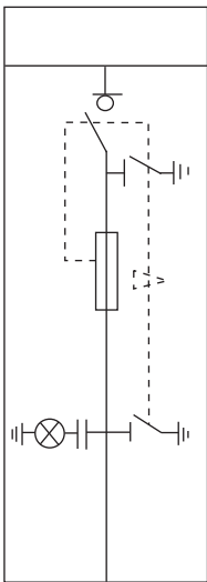
Cubicle with Switch-Fuse Combination (with SF6 Insulated Switch Disconnector)
