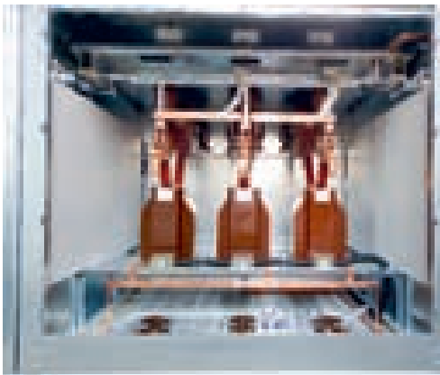
Cable Connection Compartment (At the back side of the cubicle)
