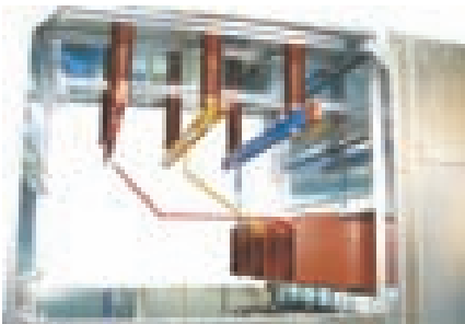
Main busbars compartment
